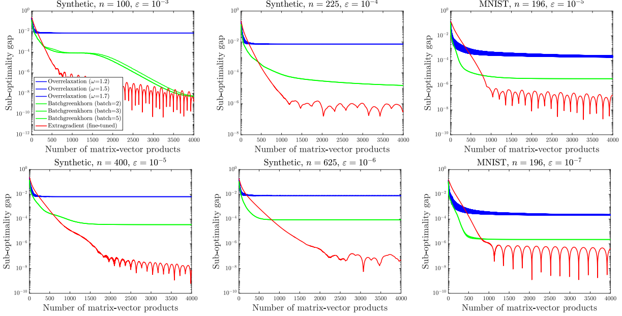
Figure 5: Empirical comparisons of our extragradient method and two cost-free acceleration strategies, namely, the overrelaxation method Lehmann et al. (2021) and the batching Greenkhorn method Kostic et al. (2022) . Each curve represents an average over 10 independent trials.
